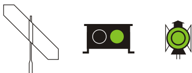
Lined for main track or lead
