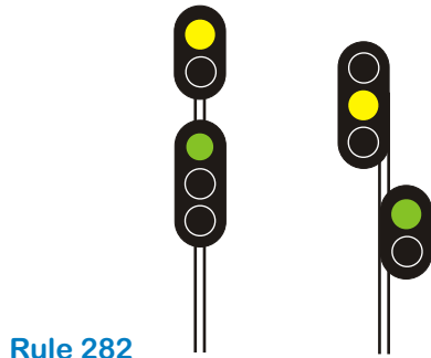
Rule 282 Indication - Proceed, Approaching Next Signal at Medium Speed
